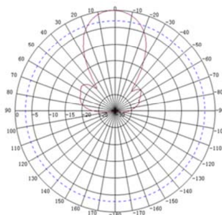
Vertical Pattern 698-960 & 1710-2700MHz
