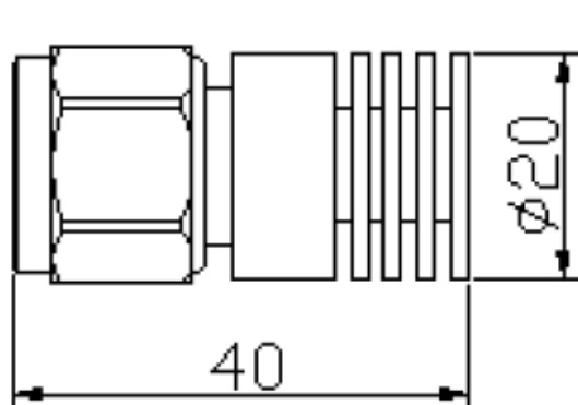
TE-2W-3GNM (Round type)
