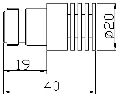
TE-2W-3GNF (Round type)
