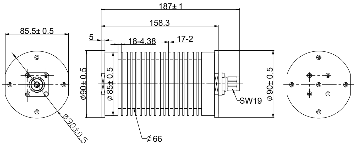
Product Drawing
