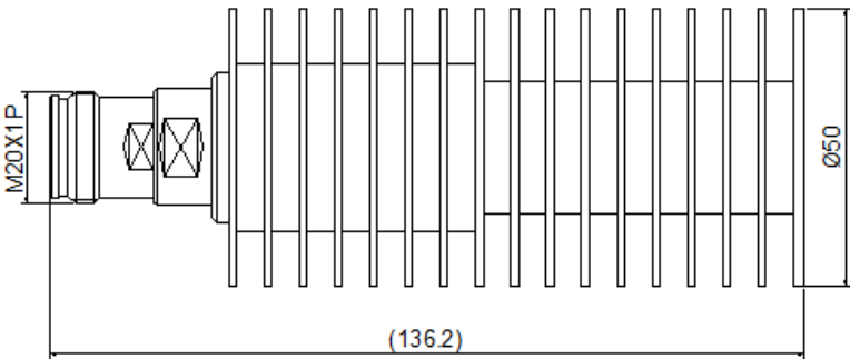
4.3-10/ Male
