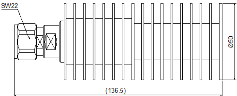
4.3-10/Female
