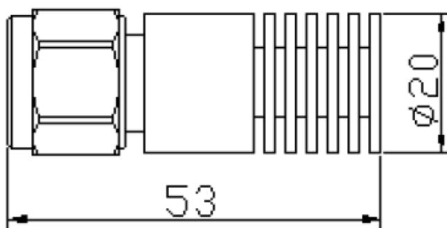
TE-5W-3GNM (Round type)
