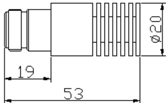
TE-5W-3GNF (Round type)
