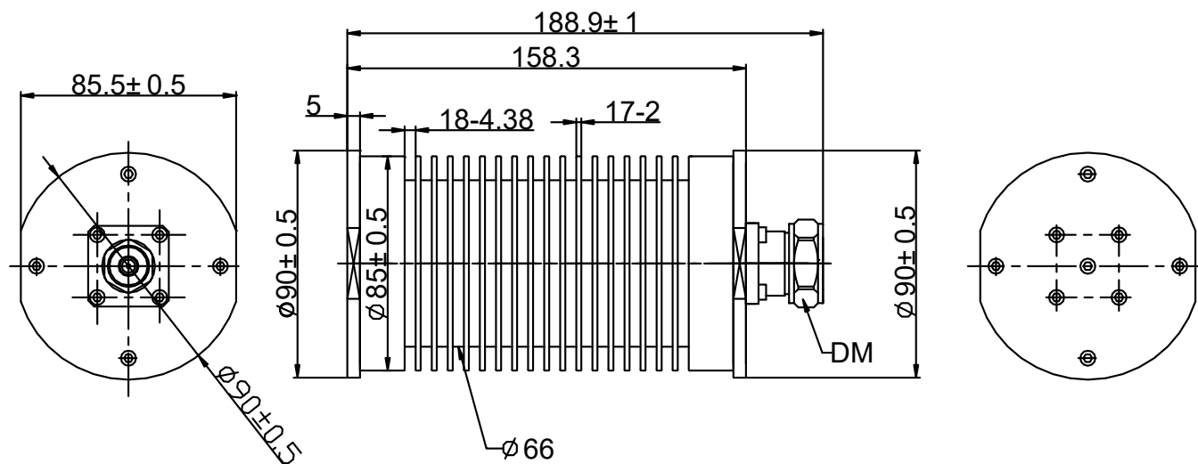
Product Drawing
